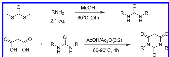
Scheme 1. Parallel Synthesis of PYTs
