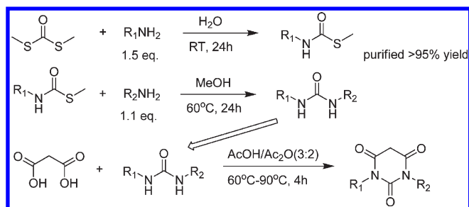
Scheme 2. Synthesis of PYT Analogues with Different R 1 and R 2 Groups
