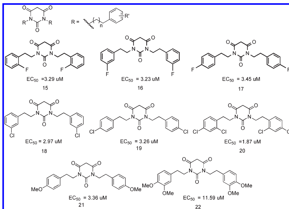
Figure 3. PYT analogues with different substituted groups on the Ph rings.
